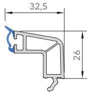
7653 - Double Glazing Bead - 28mm
