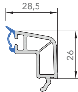
7654 - Double Glazing Bead - 32mm
