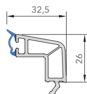
7653 - Double Glazing Bead - 28mm
