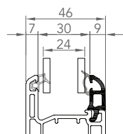
7464 PARCLOSE TRIPLE VITRAGE 24mm
