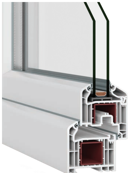
Ouvrant arrondi 3D
