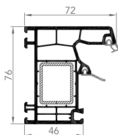
7601AE DORMANT
