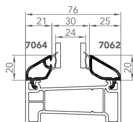
7064-7062 PARCLOSE DOUBLE VITRAGE 24mm
