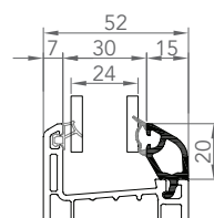
7063 PARCLOSE DOUBLE VITRAGE 24mm
