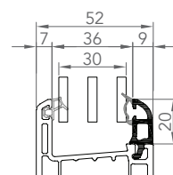
7464 PARCLOSE TRIPLE VITRAGE 30mm
