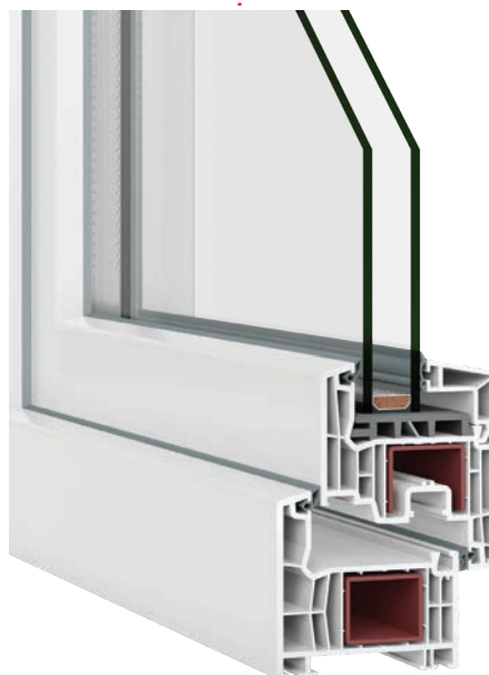
Ouvrant arrondi 3D
