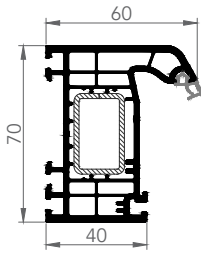
FRAME
