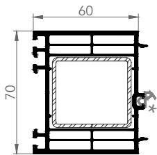
7281 70x60 mm EXTENSION
