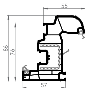
7626AE DROPPER SASH
