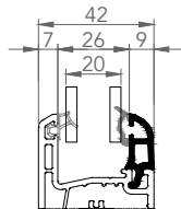
7464 DOUBLE GLAZING BEAD 20mm
