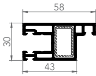
7408 SLIDING SASH PROFILE SCREENING
