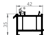
7257 FRAME EXTENSION
