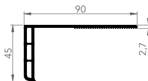
6055 MASKING PROFILE
