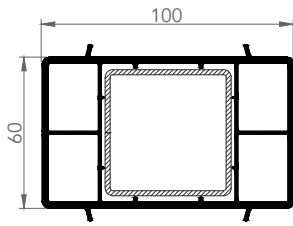
6051 60x100 BOX PROFILE
