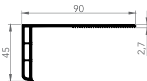
6055 MASKING PROFILE
