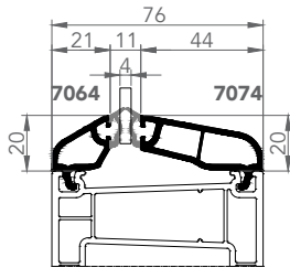
7074-7074 SINGLE GLAZING BEAD 4mm
