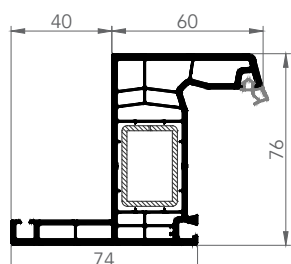
7617E RENOVATION FRAME
