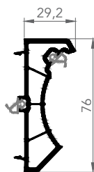
7661 CORNER ADAPTER
