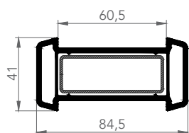
6013 WIDE SCREEN
