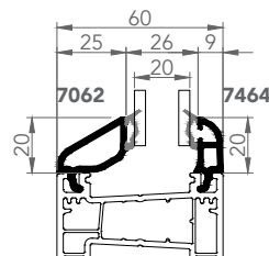
7062-7464 DOUBLE GLAZING BEAD 20mm
