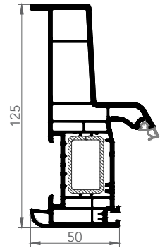
FRENCH FRAME
