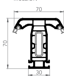
MULLION
