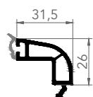
7652 DOUBLE GLAZING BEAD 24 mm
