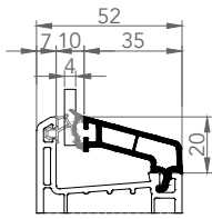
6306 SINGLE GLAZING BEAD 4mm
