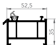
7666 FRAME EXTENSION
