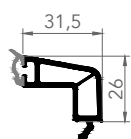
7651 DOUBLE GLAZING BEAD 24mm
