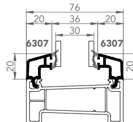
6307-6307 DOUBLE GLAZING BEAD 30mm
