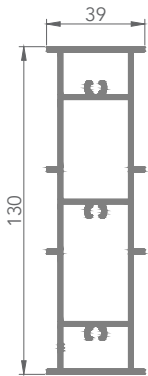
AB02005 ALUMINIUM REINFORCEMENT FRAME (6767)
