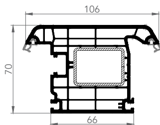
OUTWARD OPENING DOOR SASH
