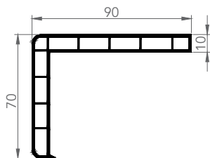
6019 MASKING PROFILE
