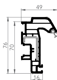
ADAPTER SASH
