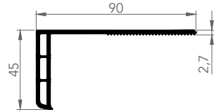
6055 MASKING PROFILE
