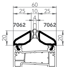
7062-7062 SINGLE GLAZING BEAD 4mm
