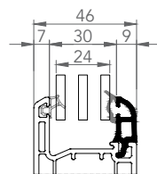
7464 TRIPLE GLAZING BEAD 24mm
