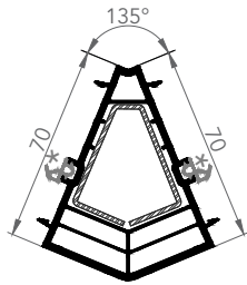
7253 CORNER PROFILE 135 DEGREES
