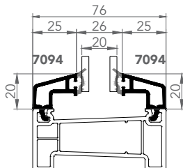
7094-7094 DOUBLE GLAZING BEAD 20mm
