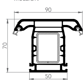
MULLION
