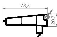
1473 FIX FRAME COVER
