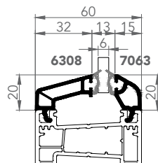
6308-7063 DOUBLE GLAZING BEAD 6mm
