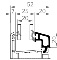
6307 DOUBLE GLAZING BEAD 20mm
