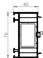
7665 76/40 EXTENSION
