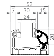
7063 DOUBLE GLAZING BEAD 24mm
