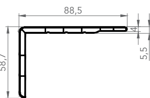
7288 MASKING PROFILE
