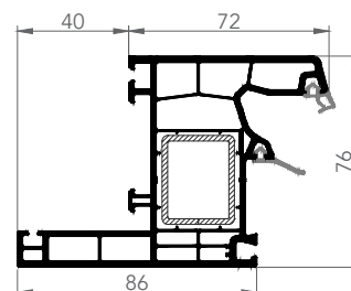
7609AE RENOVATION FRAME
