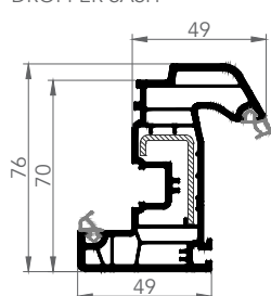
DROPPER SASH
