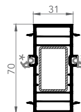
7256 CONNECTION PROFILE
