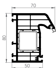
FRAME
