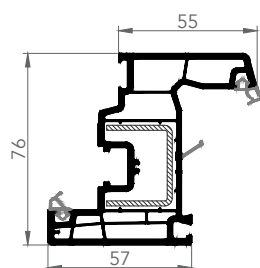
7621AE SASH
