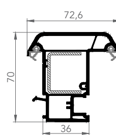
REBATE REVERSER
