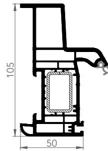
FRENCH FRAME
