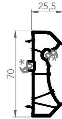
7255 CORNER ADAPTER PROFILE
