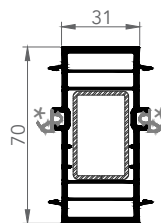
7256 CONNECTION PROFILE
