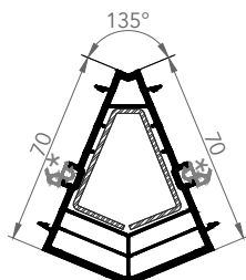
7253 CORNER PROFILE 135 DEGREES
