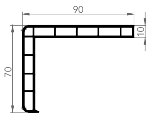
6019 MASKING PROFILE
