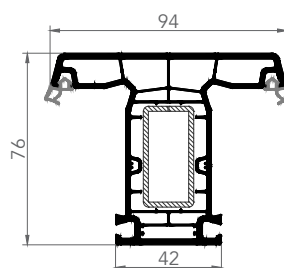
7637AE MULLION
