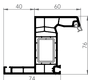
7616AE RENOVATION FRAME
