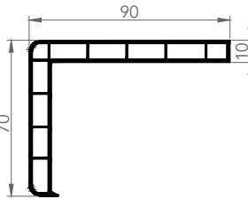
6019 MASKING PROFILE
