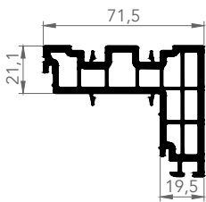
1703 INNER SILL COVER
