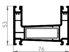
SLIDING FRAME
