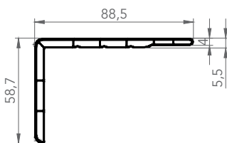
7288 MASKING PROFILE
