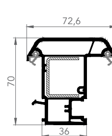
REBATE REVERSER
