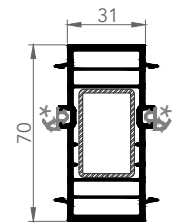
7256 CONNECTION PROFILE
