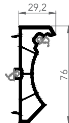
7661 CORNER ADAPTER
