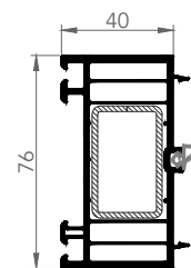
7665 76/40 EXTENSION
