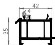
7257 FRAME EXTENSION
