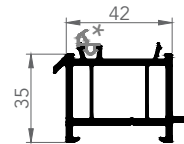
7257 FRAME EXTENSION
