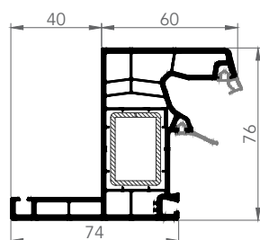
7606AE RENOVATION FRAME
