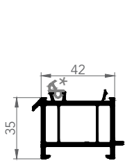
7257 FRAME EXTENSION
