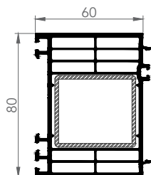
7283 80x60 mm EXTENSION
