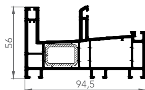
FIXED SLIDING FRAME
