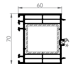
7281 70x60 mm EXTENSION
