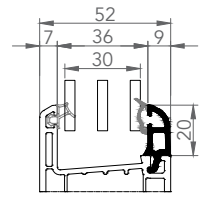
7464 TRIPLE GLAZING BEAD 30mm
