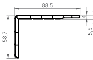
7288 MASKING PROFILE
