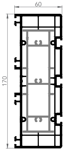
HEBE-SCHIEBE FRAME
