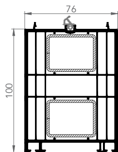
7663 76/100 EXTENSION
