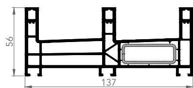
THREE-RAIL SLIDING FRAME
