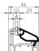
7088 DOUBLE GLAZING BEAD 4mm
