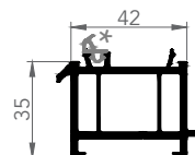
7257 FRAME EXTENSION
