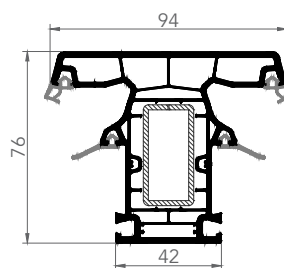
7631AE MULLION
