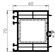
7281 70x60 mm EXTENSION
