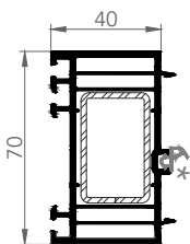
7280 70x40 mm EXTENSION
