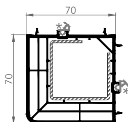
7252 70x70 CORNER PROFILE 90 DEGREES
