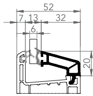
6308 SINGLE GLAZING BEAD 6-7 mm
