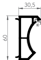
6015 CORNER ADAPTER PROFILE
