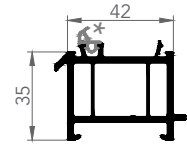
7257 FRAME EXTENSION
