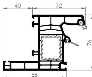
7608E RENOVATION FRAME
