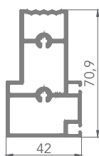
A017581 MULLION EXTENSION
