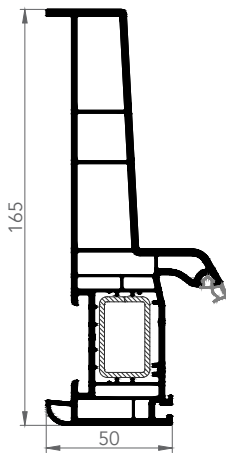
FRAME FRENCH
