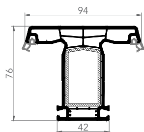
7636AE MULLION
