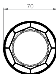
7254 CORNER PIPE
