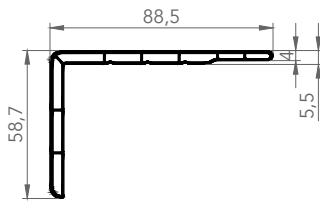
7288 MASKING PROFILE
