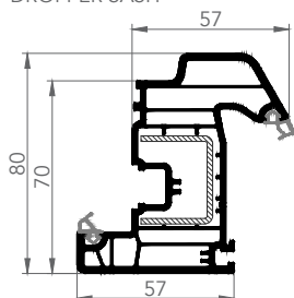
DROPPER SASH
