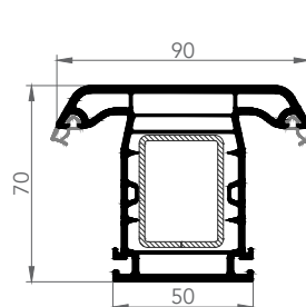
MULLION
