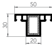
7409 SLIDING SASH in MULLION
