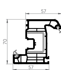
SASH
