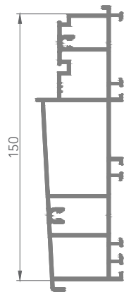
AB02001 ALUMINIUM HIGH THRESHOLD (6695)
