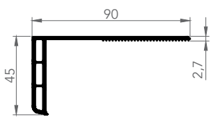
6055 MASKING PROFILE
