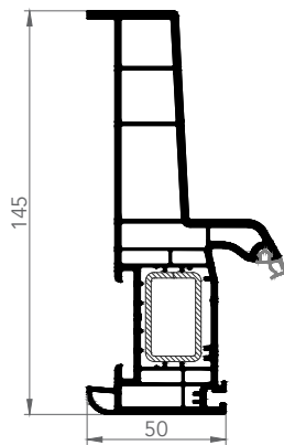
FRAME FRENCH
