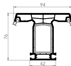
7636AE MULLION
