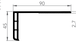
6055 MASKING PROFILE
