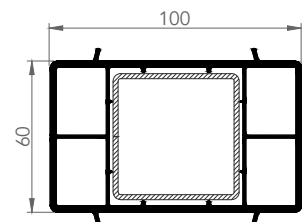
6051 60x100 BOX PROFILE
