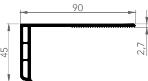
6055 MASKING PROFILE
