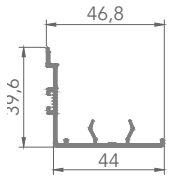
A020560 7461 SLIDING SASH ALUMINIUM INTERLOCK
