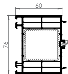
7667 76/60 EXTENSION
