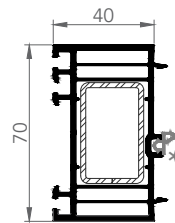
7280 70x40 mm EXTENSION
