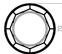
7254 CORNER PIPE
