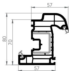
DROPPER SASH
