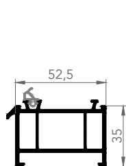
7666 FRAME EXTENSION
