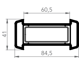
6013 WIDE SCREEN
