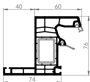
7607E RENOVATION FRAME
