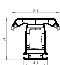
MULLION
