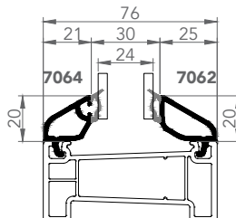
7064-7062 DOUBLE GLAZING BEAD 24mm
