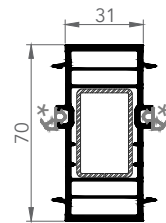
7256 CONNECTION PROFILE
