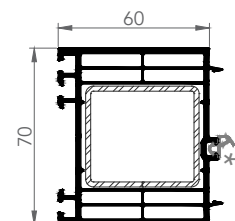
7281 70x60 mm EXTENSION
