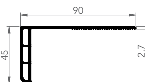
6055 MASKING PROFILE
