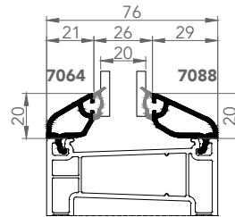
7064-7088 DOUBLE GLAZING BEAD 20mm
