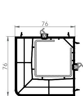
7662 90° CORNER ADAPTER
