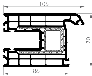
1702 HEBE-SCHIEBE SASH
