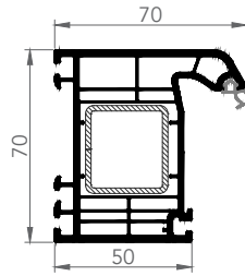
FRAME
