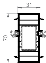
7256 CONNECTION PROFILE
