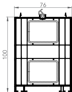
7663 76/100 EXTENSION
