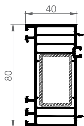
7282 80x40 mm EXTENSION
