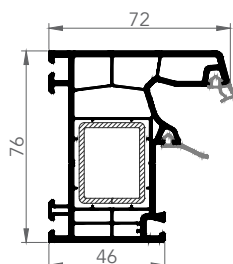
7601AE FRAME
