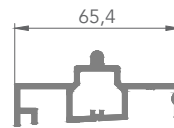
AB02007 ALUMINIUM OUTER BOTTOM RAIL LIGHT CAR (7430)
