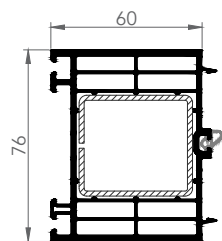
7667 76/60 EXTENSION
