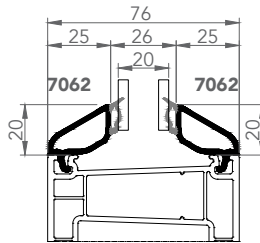
7062-7062 DOUBLE GLAZING BEAD 20mm
