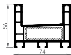
SLIDING FRAME
