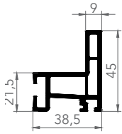
7465 SLIDING RAIL FRAME SCREENING
