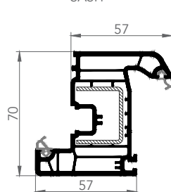
SASH
