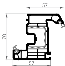
SASH
