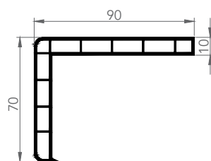
6019 MASKING PROFILE
