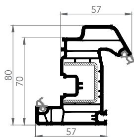
DROPPER SASH
