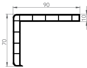
6019 MASKING PROFILE
