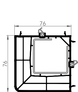
7662 90° CORNER ADAPTER
