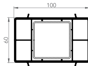
6051 60x100 BOX PROFILE
