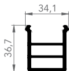
6053 FRAME EXTENSION
