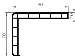
6019 MASKING PROFILE
