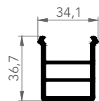
6053 FRAME EXTENSION
