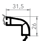
7652 DOUBLE GLAZING BEAD 24mm
