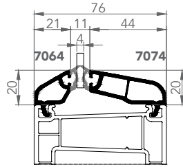
7074-7074 TEK CAM ÇİTASI 4mm
