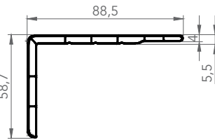
7288 İNCE PERVAZ
