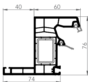
7606AE PERVAZLI KASA
