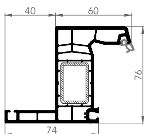
7616AE PERVAZLI KASA
