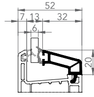
6308 TEK CAM ÇİTASI 6-7 mm
