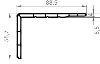
7288 İNCE PERVAZ
