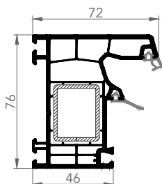
7601AE KASA
