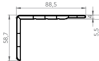
7288 İNCE PERVAZ
