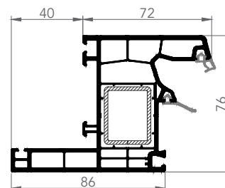
7609AE PERVAZLI KASA
