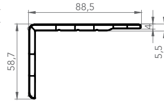
7288 İNCE PERVAZ
