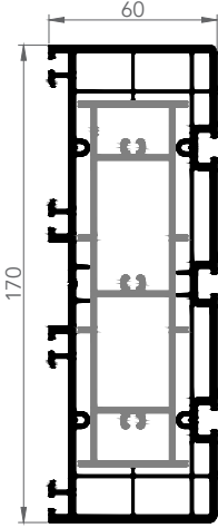
HEBE-SCHIEBE KASA
