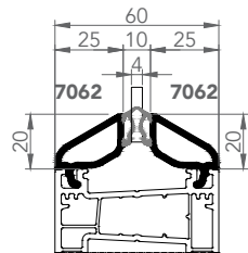
7062-7062 TEK CAM ÇİTASI 4mm
