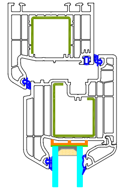
AA - DETAYI
