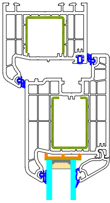
AA - DETAYI
