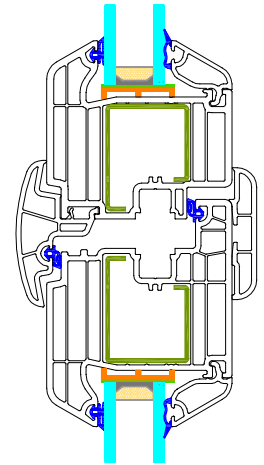
AA - DETAYI
