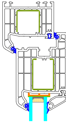
BB - Detail
