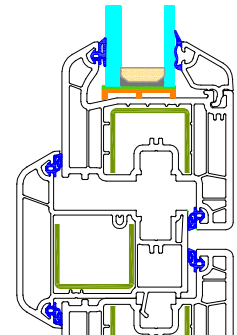
BB - Detail
