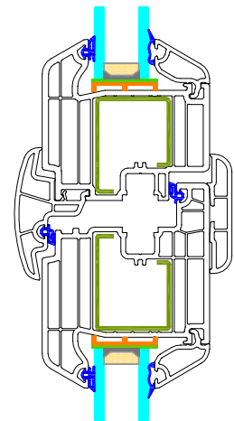
AA - Detail
