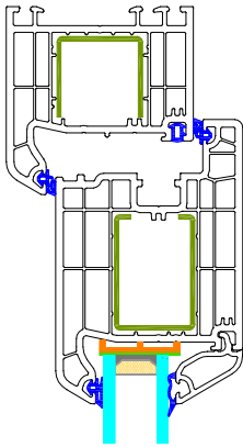
AA - Detail
