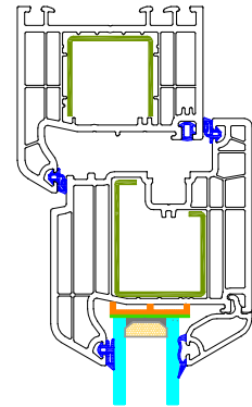
AA - Detail
