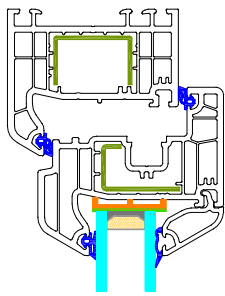
BB - Detail
