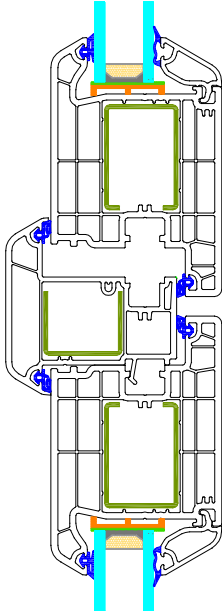
AA - Detail
